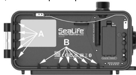
Pre-installed medium-sized rubber grip tabs (A)
